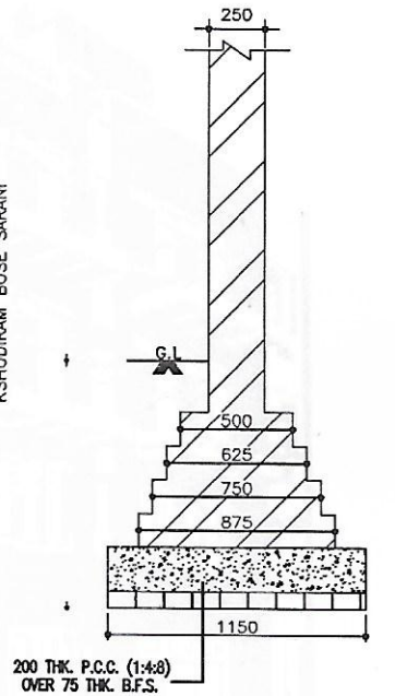
DETAILS OF EXISTING BOUNDARY WALL SCALE-1:25
